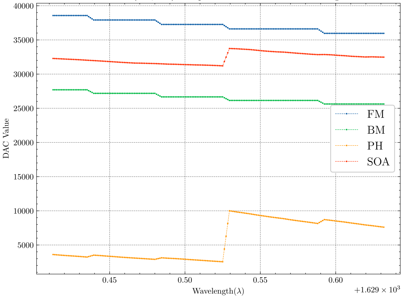
DAC Parameters (425, 475) Interpolated with 3 Intermediate Integer Values
